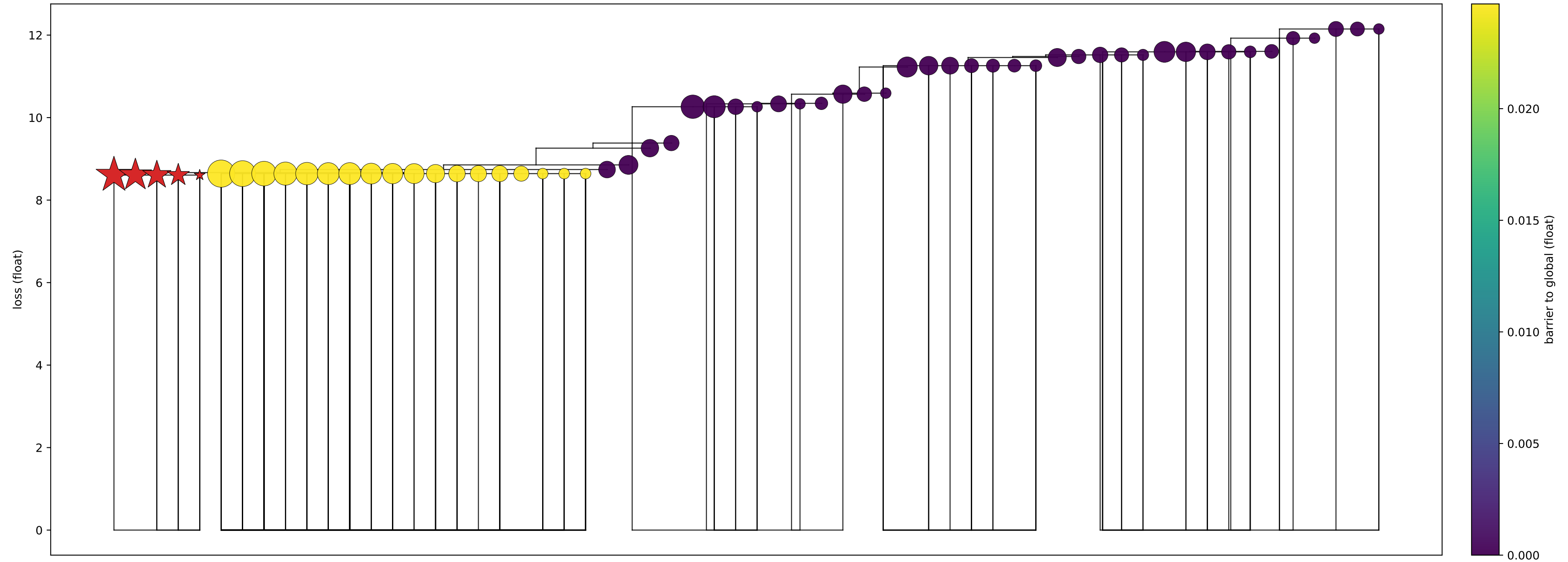
Disconnectivity tree over sinks (sublevel connectivity) p=3, n=20, d=3, loss=l1, noise=haar(k0=0,kmax=6); sinks=61 (shown=60)
